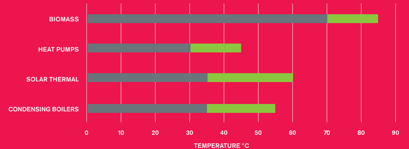
Optimum Operating Temperature Ranges For LZC Solutions
