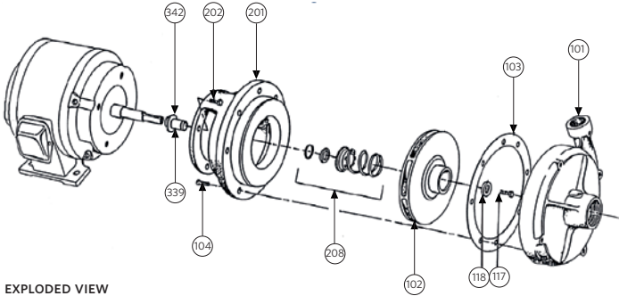
EXPLODED VIEW
